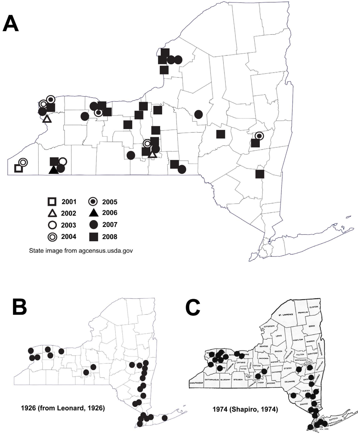
FIG. 2. Recent versus historical distribution of P. crespontes sightings in New York State.
