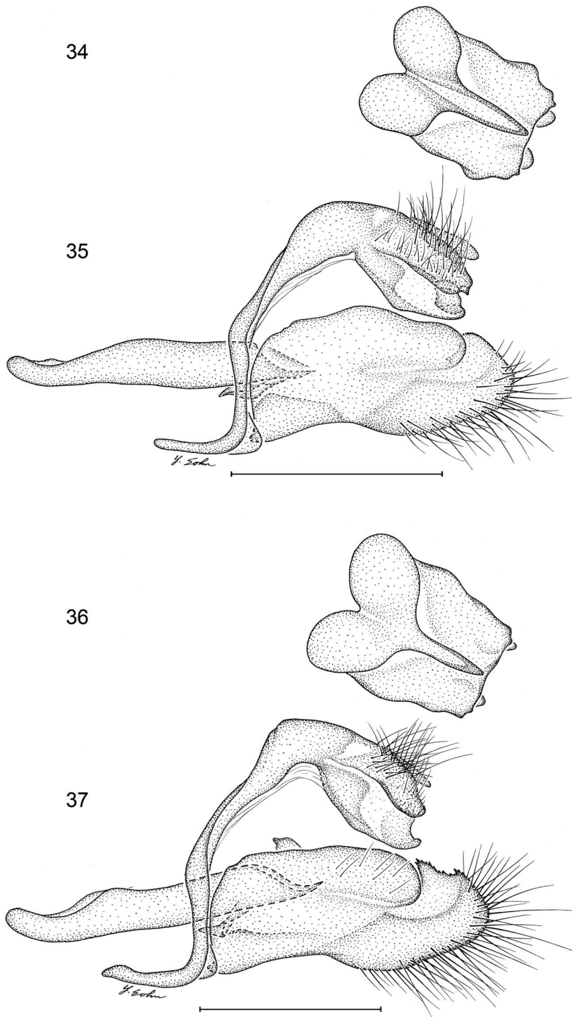
FIGS. 34–37. Male genitalia of two species of Cobalus from ACG, Costa Rica (USNM), scale = 1.0 mm. 34, 35 , C. virbius , X-5873, 99-SRNP-6213. 36, 37 , C. fidicula , X-5876, 99-SRNP-5803. 34, 36 , Tegumen, uncus, and gnathos in dorsal view. 35, 37 , Complete genitalia in left lateral view.
