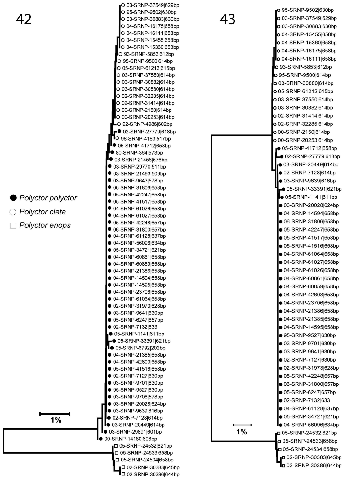
FIGS. 42, 43. Neighbor-joining (NJ) trees based on Kimura-2-Parameter (K2P) distances for cytochrome c oxidase I (COI) of Polyctor from ACG, Costa Rica. Outgroup, P. enops . Rearing voucher code and sequence length given for each individual. To find the larval foodplant of any individual, enter its voucher code in the ACG database (Janzen & Hallwachs 2006). 42 , 19 P. cleta and 44 P. polyctor with various COI sequence lengths. 43 , 17 P. cleta and 35 P. polyctor with COI barcodes of sufficient lengths (approaching or exceeding 650 base pairs) for distinguishing these species.
