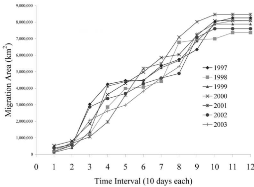
FIG. 4. Plot of the increase in area (km 2 ) occupied by the monarch migration in each 10-day interval for each year. Intervals begin on 1 March and end on 28 June.
