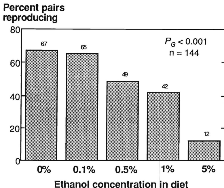
FIG. 2. Fertility or reproductive fraction of pairs of Choristoneura fumiferana adults receiving different ethanol concentrations for imbibing. Results for the two experiments with different diet bases are pooled.
