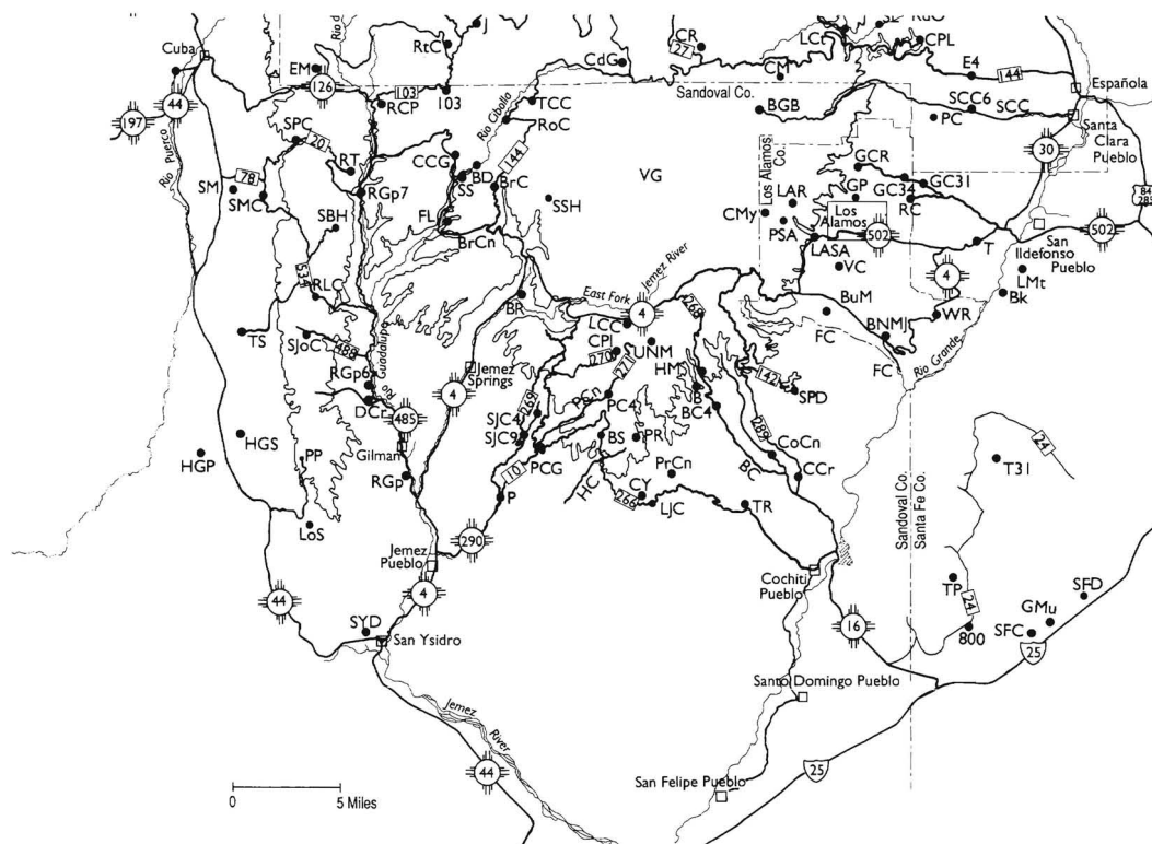
FIG. 2. Jemez Mountains, New Mexico, collecting sites (southern portion) and 8000' elevation contour. Same scale as Fig. 1.
