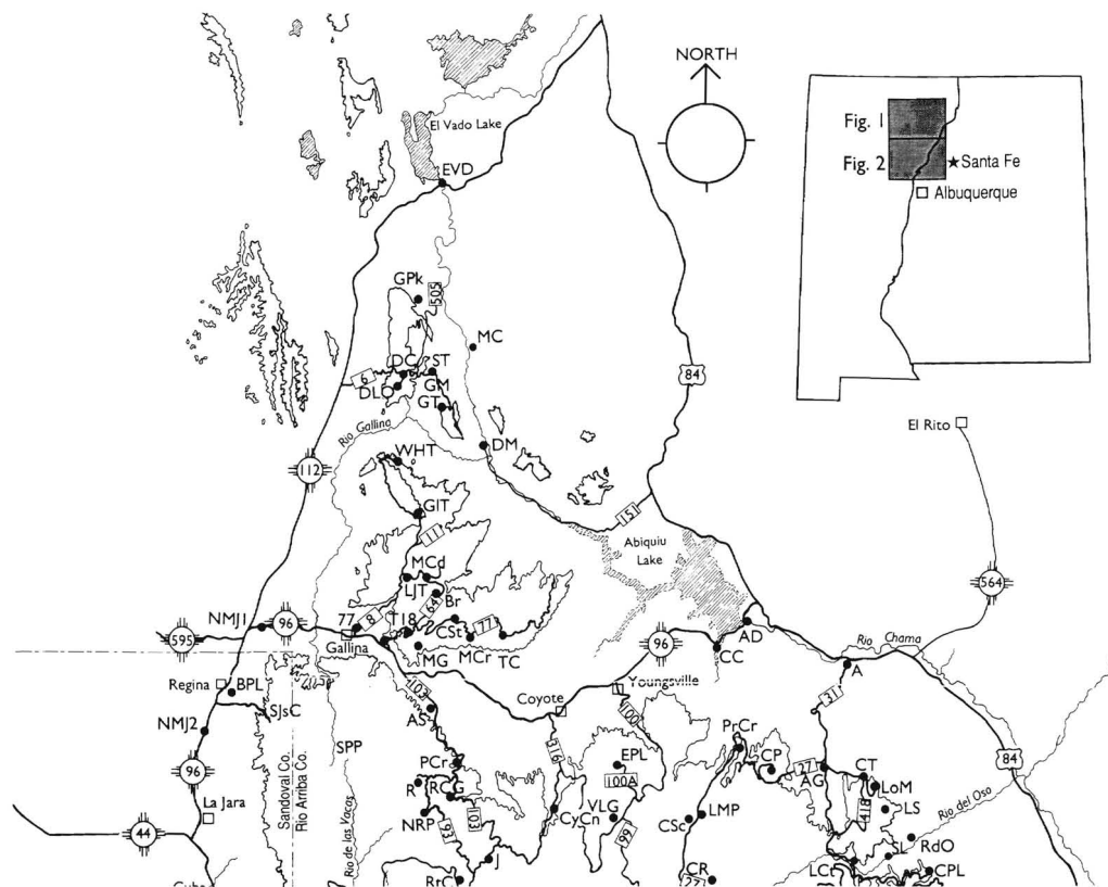
FIG. 1. Jemez Mountains, New Mexico, collecting sites (northern portion) and 8000' elevation contour. Same scale as Fig. 2.
