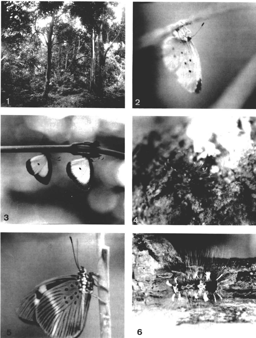
FIGS. 1-6. 1, Cola forest habitat, Agbara, Lagos, Nigeria. The taller trees are Cola nitida ; 2, Pentila bitje ovipositing on a dead branch; 3, Liptena opaca feeding on extrafloral nectaries of a creeper; 4, Third instar larva of Larinopoda aspidos feeding on epiphylls; 5, Male Aethiopana honorius resting on bamboo stem; 6, Larva of A. honorius . Note long lateral setae.
